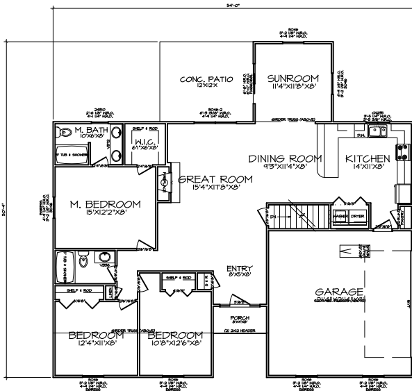
1 FIRST FLOOR PLAN A-4
