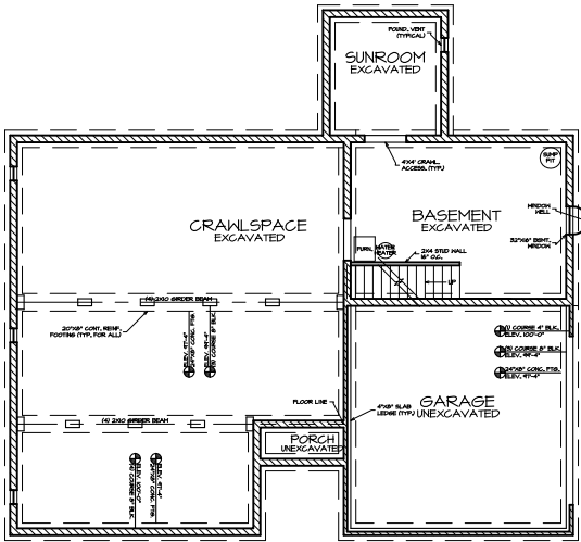
1 FOUNDATION PLAN A-3
